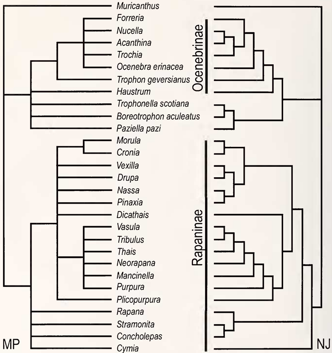
Figure 54. Strict consensus maximum parsimony [MP] and neighbor-joining [NJ] trees depicting the relationships of genera based on data derived from their type species. Data from Kool (1993b:Table 3) have been supplemented by data for Ocenebra erinacea , Trophon geversianus , Trophonella scotiana , Boreotrophon aculeatus , and Paziella pazi .
